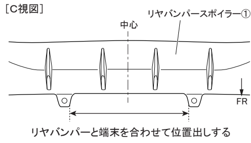
[C視図]
